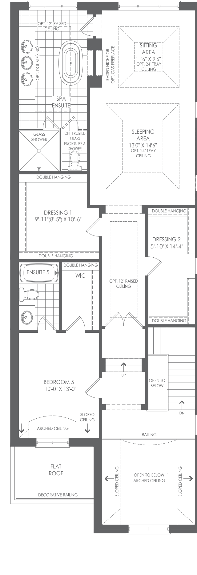
OPTIONAL THIRD FLOOR ELEV. A 5 BEDROOM PLAN
